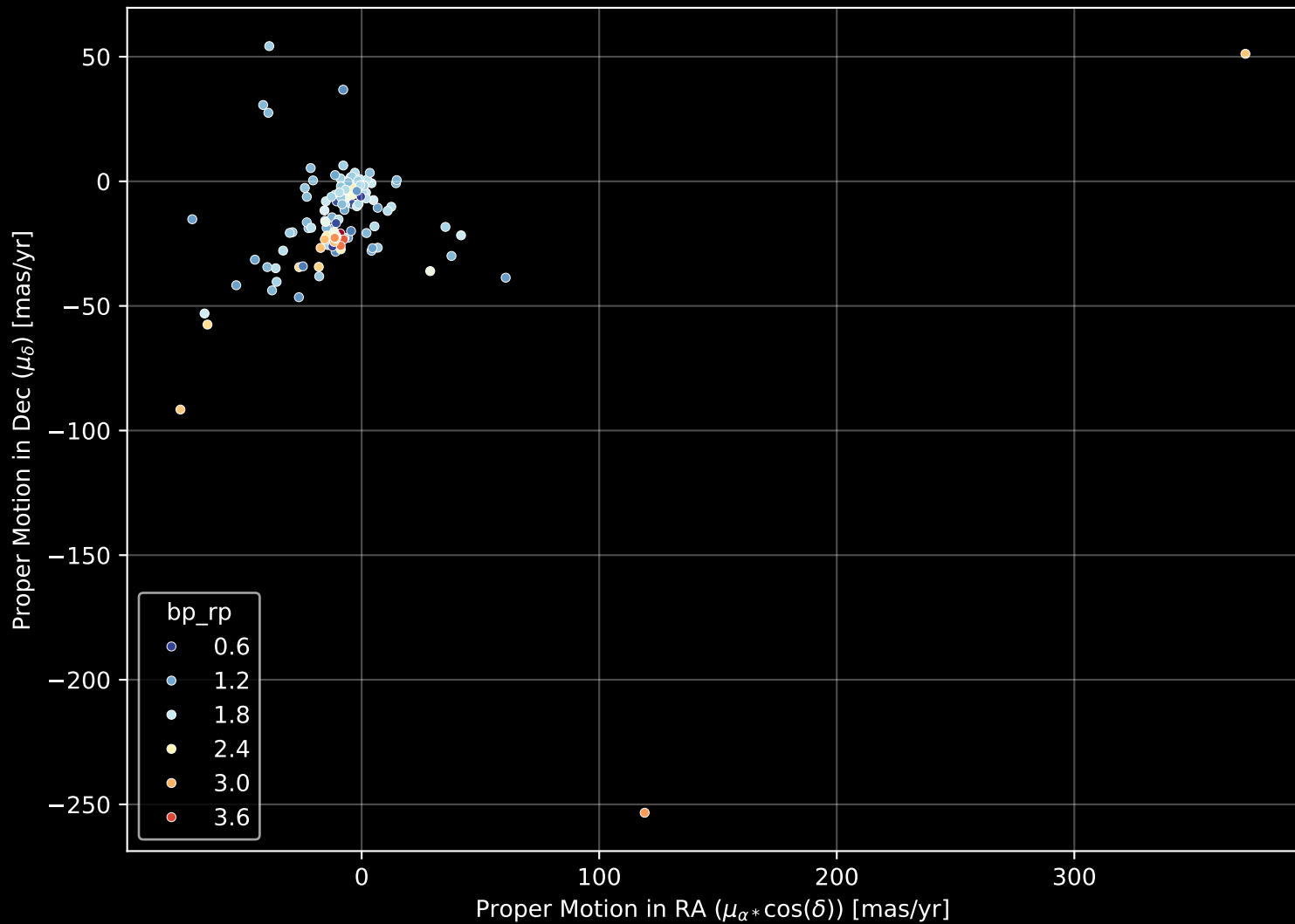
APOGEE DR17 Field: [350+18-O] Proper Motion Diagram (n= 141)
