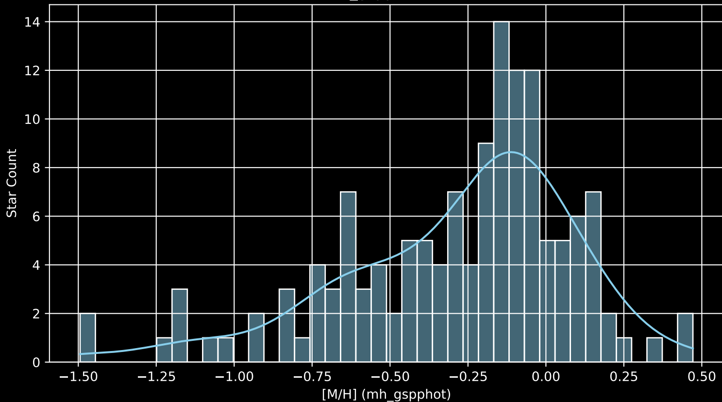
APOGEE DR17 Field: [350+18-O [M/H] (mh_gspphot) (n= 138)
