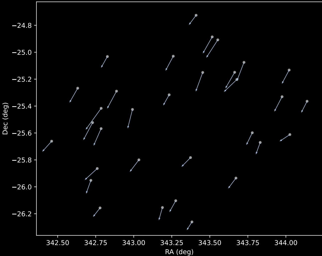
APOGEE DR17 Cluster 1 Proper Motion Vectors (n=32)
