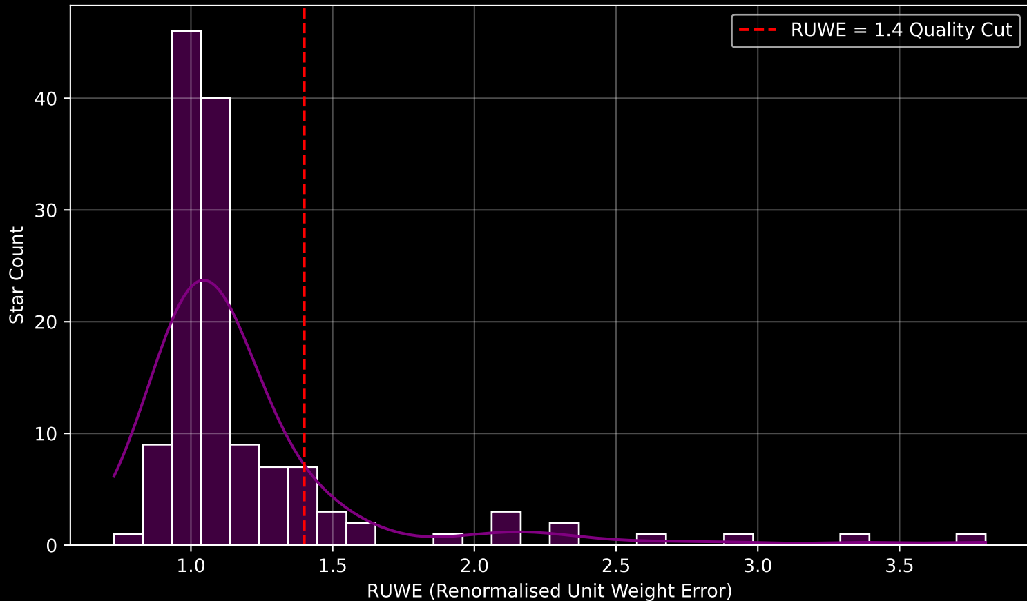
GAPOGEE DR17 Field [350+18-O] RUWE Distribution (n= 134)
