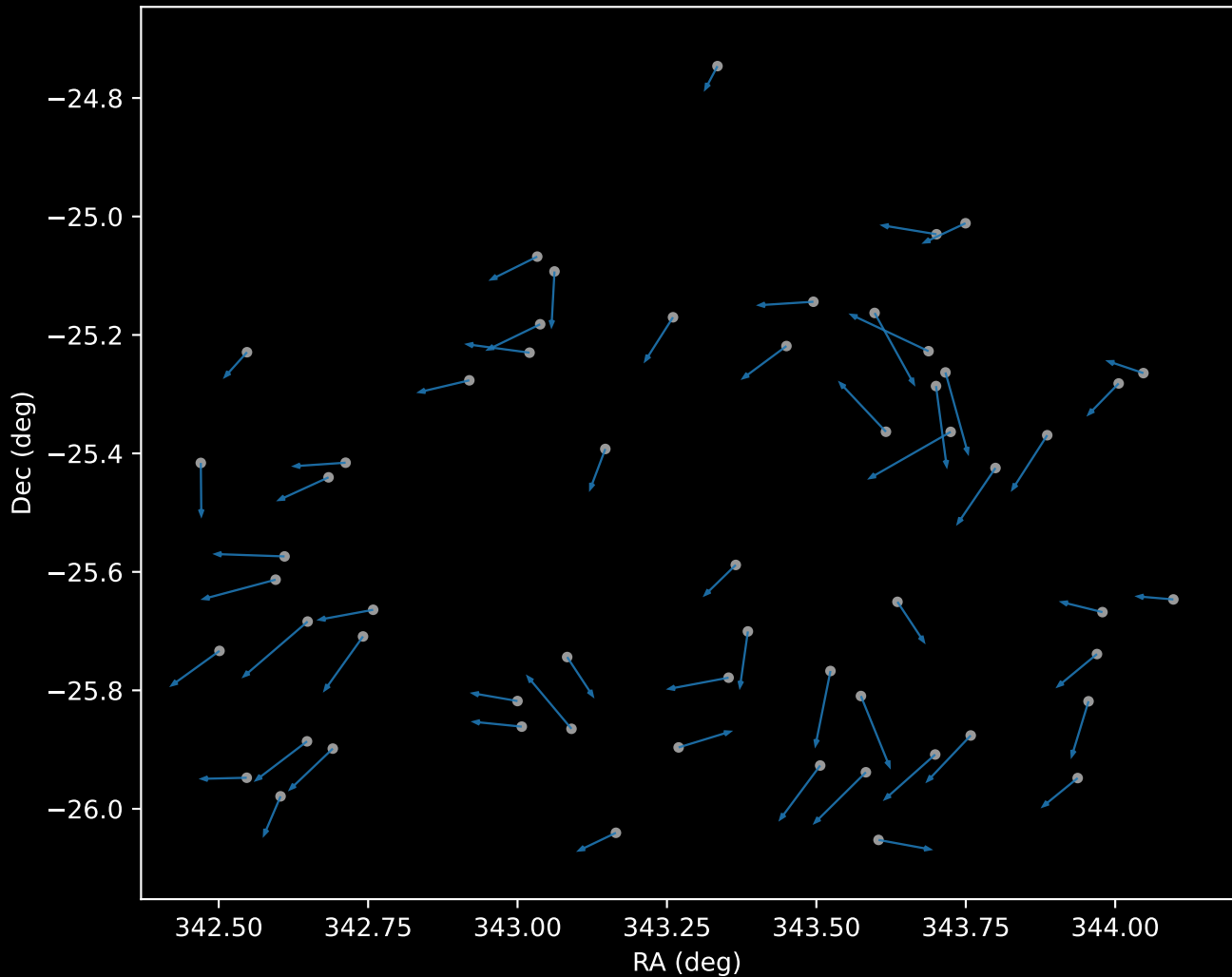
APOGEE DR17 Cluster 0 Proper Motion Vectors (n=58)
