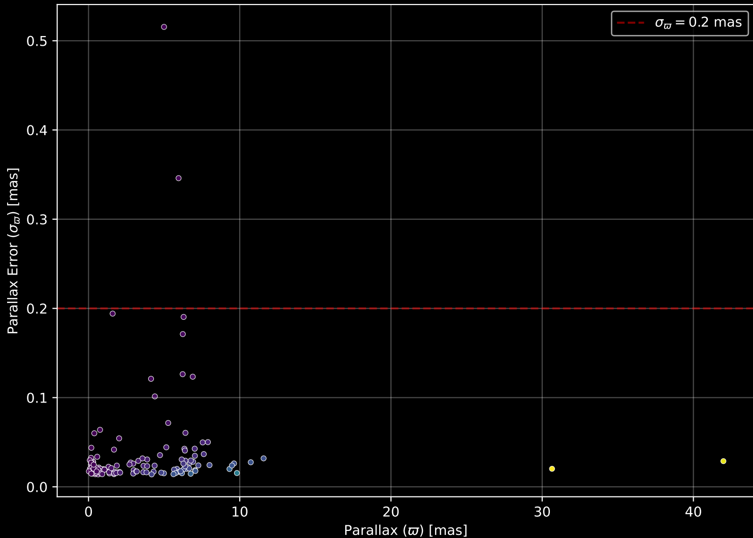
APOGEE DR17 Field: [350+18-O] Parallax Quality (n= 141)
