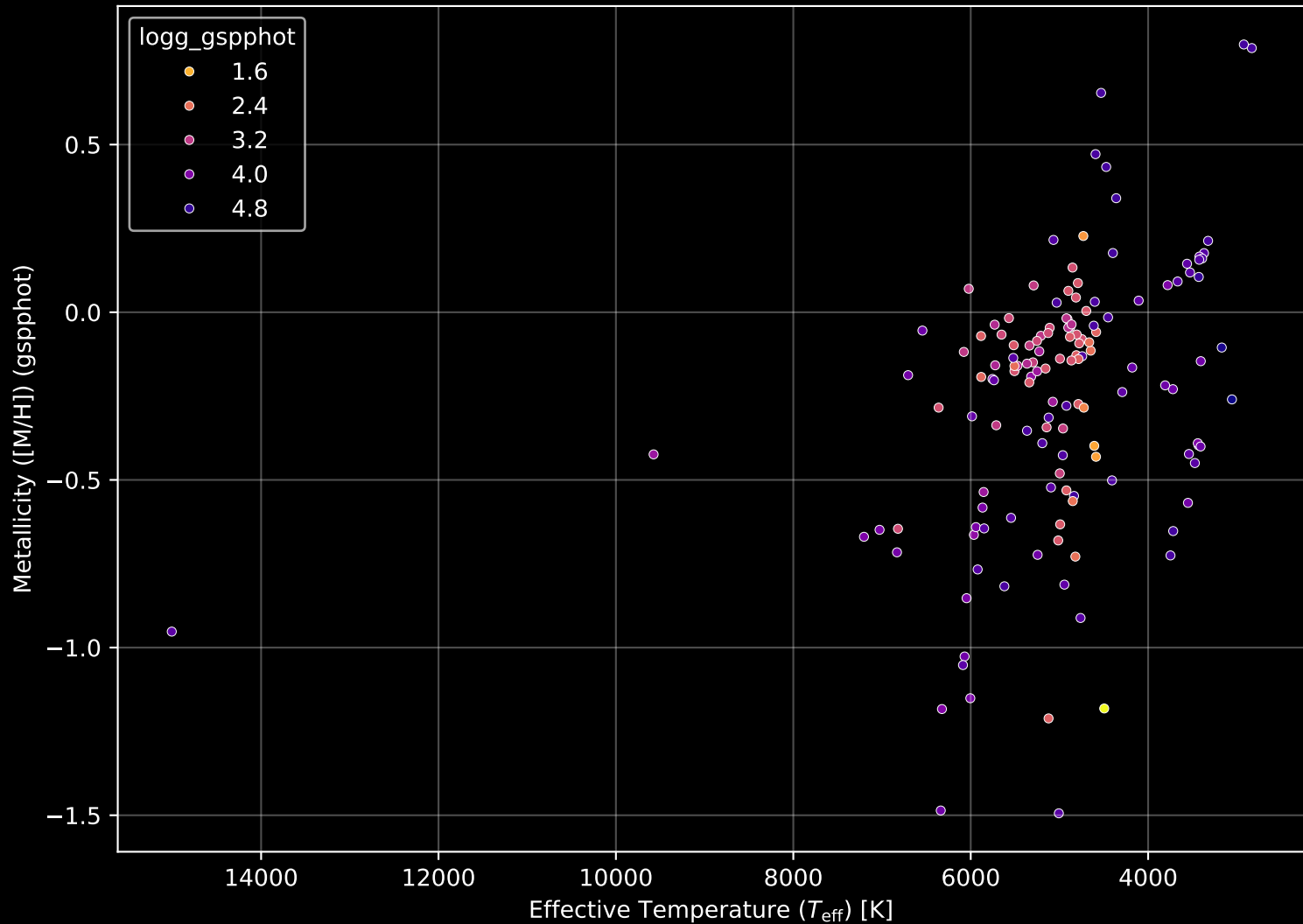
APOGEE DR17 Field: [350+18-O] Stellar Population Parameters (n= 141)
