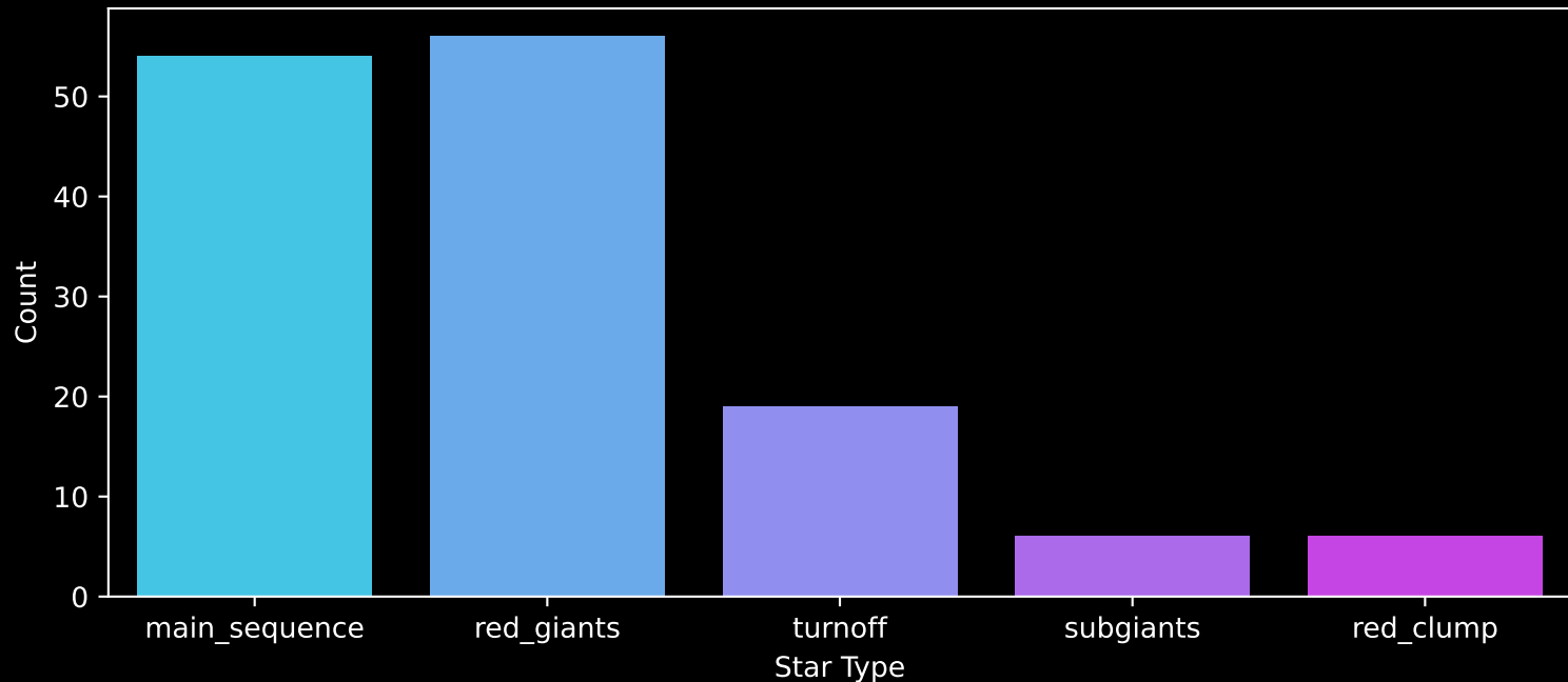
APOGEE DR17 Field: [350+18-O] Count plot of Star Type
